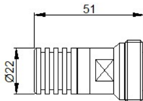
2W/5W 7/16 Female
