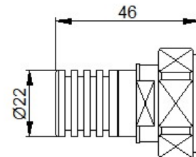
2W/5W 7/16 Male
