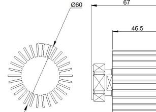
10W/25W 7/16 Male
