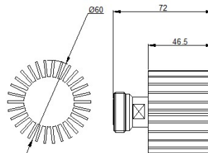
10W/25W 7/16 Female
