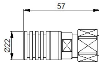
2W/5W 4.3-10 Male
