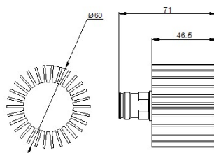
10W/25W 4.3-10 Female
