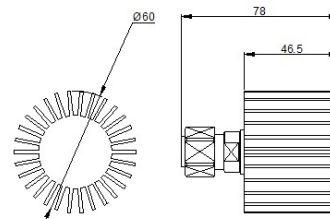
10W/25W 4.3-10 Male
