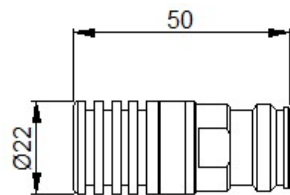
2W/5W 4.3-10 Female
